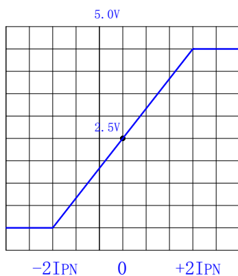
Current ( I_P ) - Output ( V_0 )
